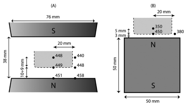
FIGURE 2. Illustrations of magnetic field configurations used in the experiment. Dots and adjacent numbers represent the measured vertical magnetic field strength (in mT). The light-gray area denotes the volume occupied by the magnetic suspension, and the horizontal dashed line indicates the location of the substrate: (A) a relatively homogeneous magnetic field created by the electromagnet with circular poles; (B) a strongly inhomogeneous field created by the cubic NdFeB magnet. Notice that the third dimension of the permanent magnet is the same as the other two and that the magnetic suspension is placed in the center of the upper square plane of the magnet.
