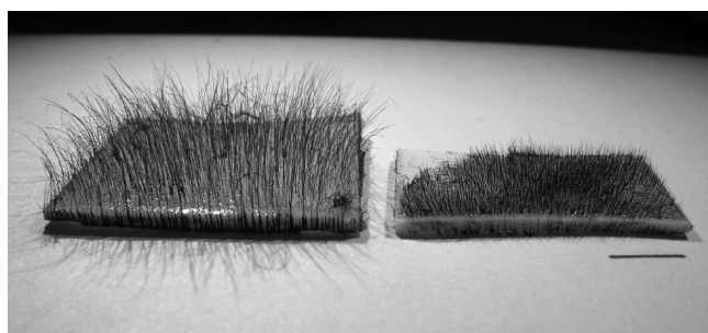
FIGURE 3. Photograph of two PTFE substrates covered with magnetic cilia mimics made in a magnetic field of 450 mT with a vertical gradient of 0.1 T/m using the electromagnet (left) and with a vertical gradient of 20 T/m using the permanent magnet (right). The scale bar is 5 mm.
