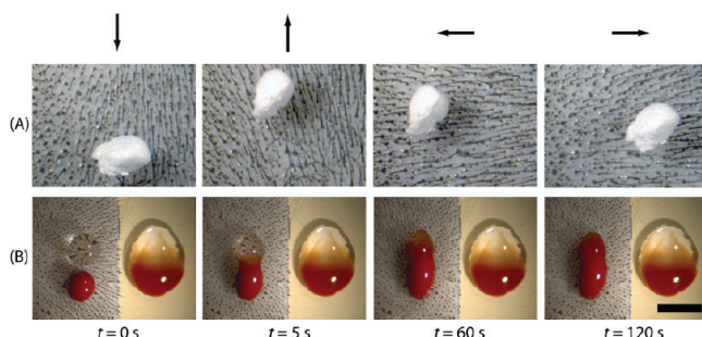
FIGURE 6. Optical micrograph sequences demonstrating actuation and mixing with the magnetic cilia. (A) Magnetic cilia as an actuator inducing movement to a 3 mm piece of expanded polystyrene. Arrows indicate the magnetic field direction. (B) Mixing of two drops of glycerol (one clear and one stained red) by periodic actuation of the magnetic cilia mimics at a rate of 1–2 beats/s (left) compared to diffusive mixing (right) at different time intervals. The scale bar is 5 mm. Videos are available in the Supporting Information.
