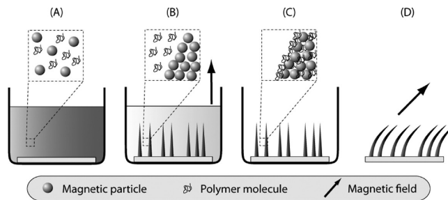
FIGURE 1. Schematic illustration of the structure formation in a dilute magnetic suspension: (A) the initial mixed state (no magnetic field); (B) the phase-separated state (magnetic field perpendicular to the substrate); (C) the solvent removed state (no magnetic field); (D) the functional state (magnetic field in an arbitrary angle).
