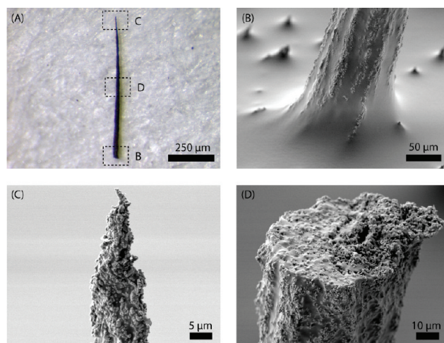
FIGURE 4. (A) Optical micrograph of a typical single magnetic cilium with an aspect ratio of 28. Marked areas (B–D) are shown magnified in the scanning electron microscope images: (B) the cilium base; (C) the cilium tip; (D) the cilium cross section.
